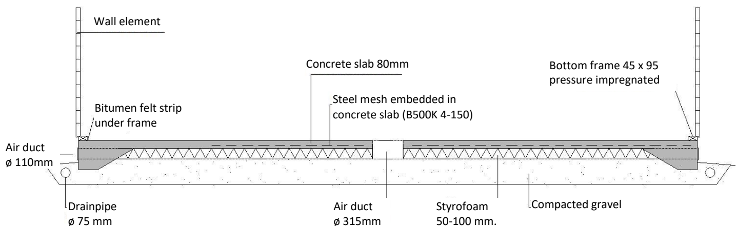
Foundation Section A-A
