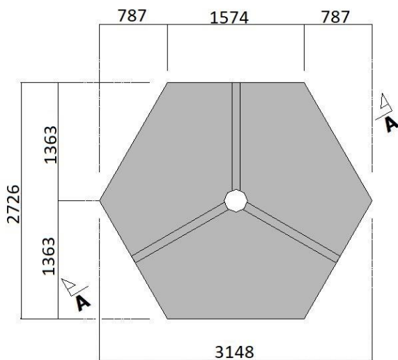
Foundation drawing
