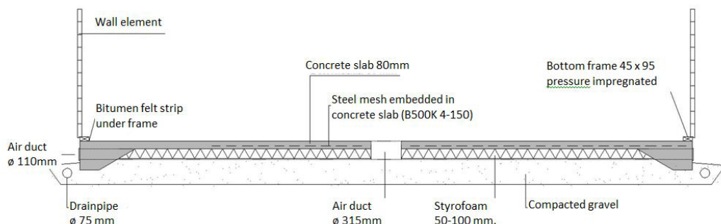
Foundation Section A-A
