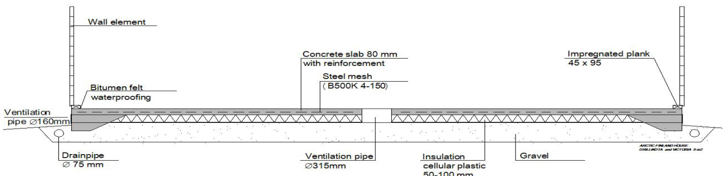
Foundation, section A - A :
