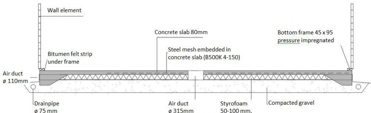
Foundation Section A-A
