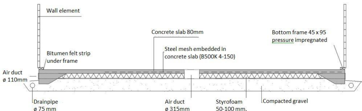
Foundation Section A-A
